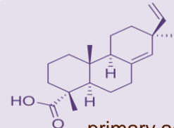
primary acid 6
